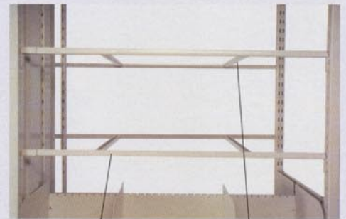
Longitudinal Support Shelf Reinforcement
