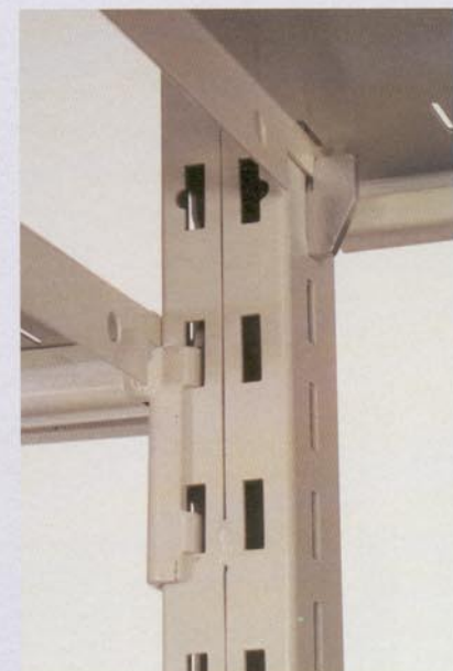
Two technologies in a single post-frame
